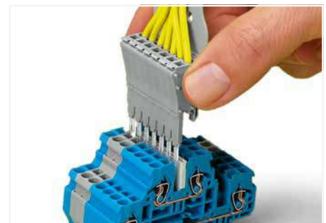
Testing is also possible using a pre-wired tap-off module assembly in the very same way as test plugs.
