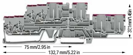
4-conductor/4-pin double-deck carrier terminal block; 4-conductor/4-pin through terminal block; internally commoned; Violet conductor entry; gray
