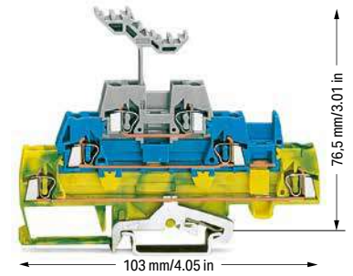
Triple-deck terminal block; ground conductor/through/through terminal block
