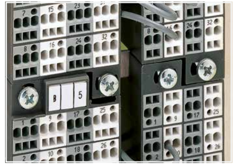
Space saving: Slimline matrix patchboard (lower right), mounted upside down
