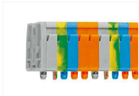
Terminal strips with snap-in mounting feet; for 0.6 ... 1.2 mm plate thickness; mounting holes: 3.5 +0.1 mm Ø
