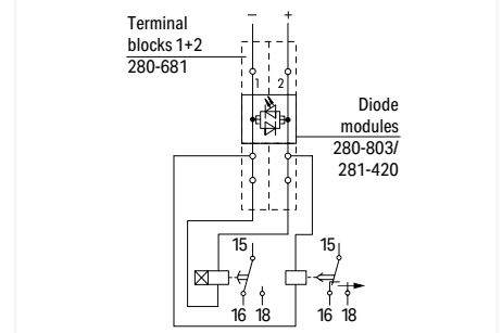
Free-wheeling diode and voltage check
