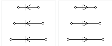
Triple-deck diode terminal block; with three 1N4007 diodes; gray
