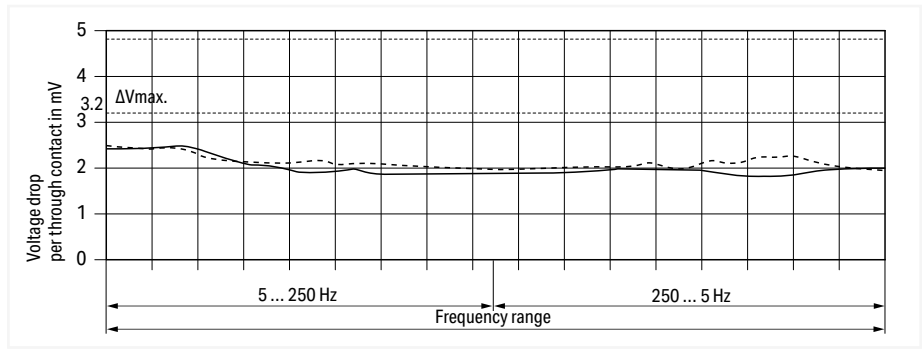
Frequency cycle: 5 ... 250 Hz, 250 ... 5 Hz Rail-mount terminal block: Item no. 280-681 Test current: 1/10 I N = 2,4 A ----- Test specimen no. 1 - - - - - Test specimen no. 2
