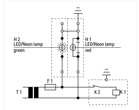
Operating condition Slide link closed, auxiliary circuit grounded, green LED/neon lamp illuminates.
