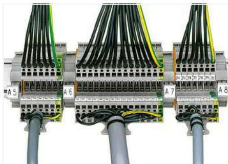
Cable entry into the control cabinet: The cables are led into the control cabinet with the connected female plugs and are directly plugged onto the carrier terminal blocks.
