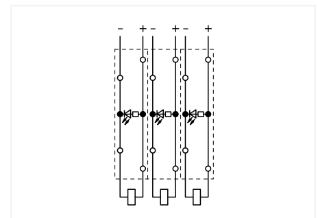
Circuit-related voltage indications can be created using the following terminal blocks: 870-543/281-434 or 870-543/281-413
