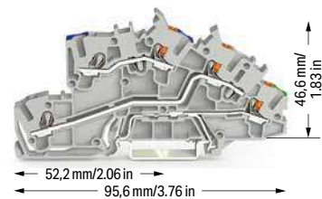
Multilevel installation terminal block; with operating slot and push-button; gray
