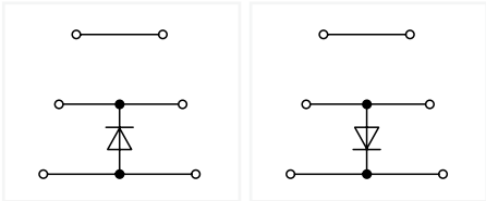
Triple-deck diode terminal block, with 1N4007 diode; gray
