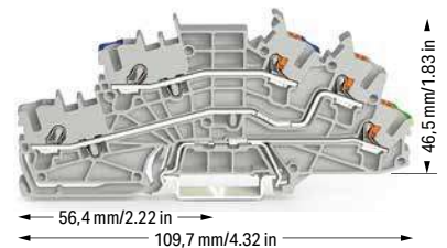
Multilevel installation terminal block; with operating slot and push-button; gray
