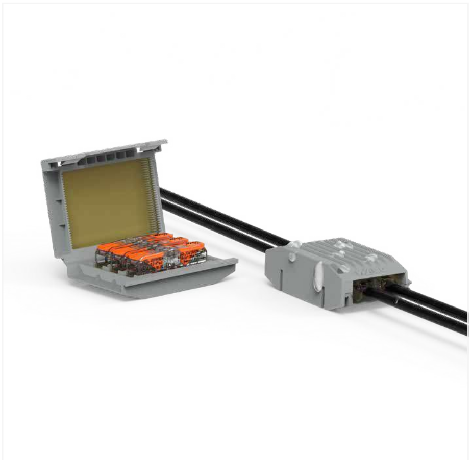
Re-accessible: Open the Gelbox, remove the gel, open the connector and rewire with new components.
