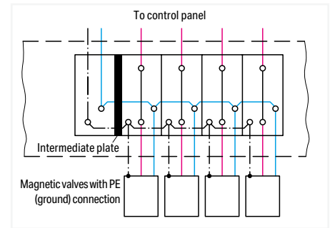
Power supply from control panel side
