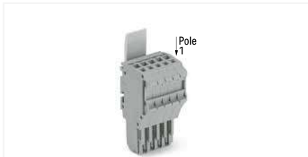
1-conductor female plugs; with locking levers and strain relief plates
