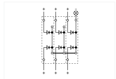
Collective fault signals can be created using the following terminal blocks: 870-541/281-489 or 870-541/281-490
