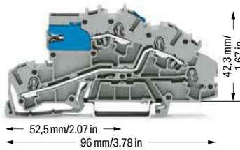
Multilevel installation terminal block; with N-disconnect slide link; gray
