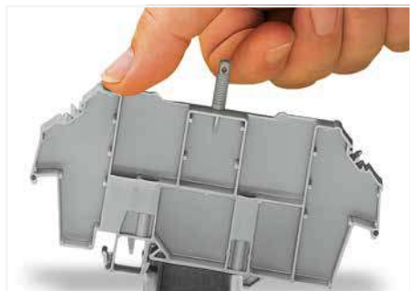
Snapping a cover carrier onto the DIN-rail.
