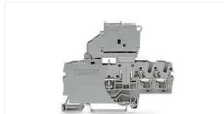
Fused disconnect terminal blocks with a pivoting fuse holder for glass cartridge fuses
