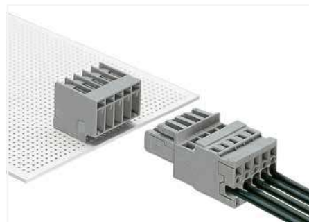
Male headers with angled solder pins (769-662 to 769-675)
