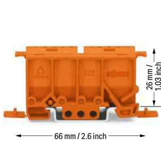
Mounting carrier; for 2-, 3- and 5-wire splicing connectors; 22 mm wide
