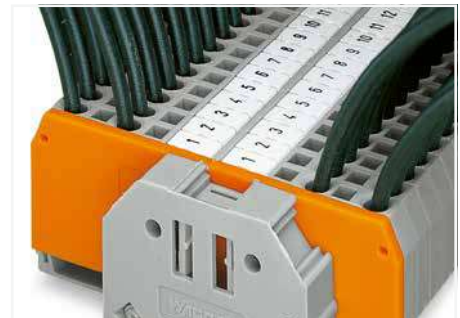
Marking directly on the terminal block via WMB markers.
