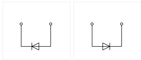
1-conductor/1-pin diode carrier terminal block; with two jumper positions
