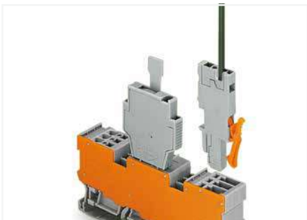
1-conductor/1-pin carrier terminal block; with two jumper positions 1-conductor female plug; straight* Fuse plug; 6 mm wide (every other terminal block) *1-conductor angled female plug is also possible!
