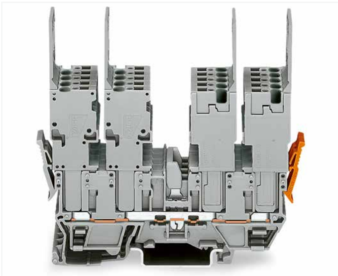
4 x 1-conductor female plugs Carrier terminal blocks can be commoned via 280 and 780 Series Jumpers and tested using a test plug adapter (280-4..).
