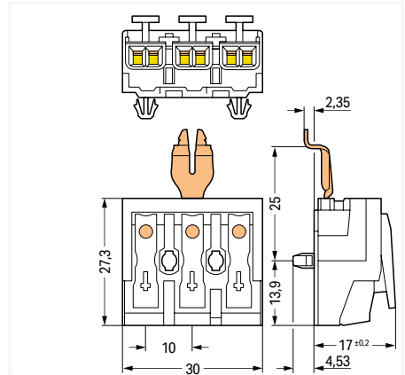
Field-wiring terminal block; with angled ground contact; with snap-in mounting feet; 3-pole; white
