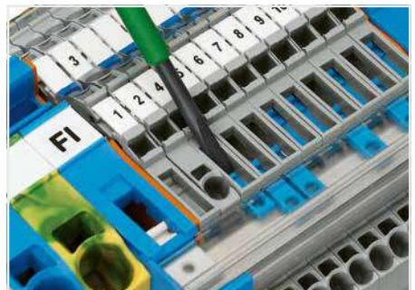
Operating a disconnect slide link with an operating tool (3.5 mm blade width) Item number (operating tool): 2009-309, 2009-310, 210-658 or 210-720
