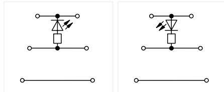
Triple-deck LED terminal block; with red LED; gray
