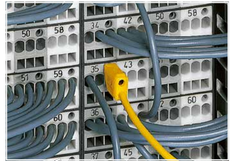
Testing with a 2.3 mm Ø test plug.
