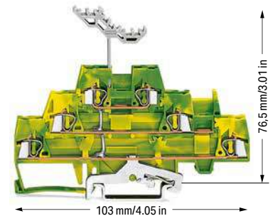
Triple-deck terminal block; 6-conductor ground terminal block; internally commoned
