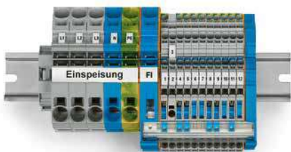
Subdistribution board set TOPJOB® S; with operating slots
