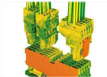
4-pin ground carrier terminal block 1-conductor female plug; straight 2-conductor female plug
