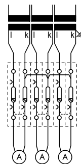
Transformer test circuit, k-conductors of the transformers connected
