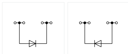
4-conductor diode terminal block; with 1N4007 diode; gray
