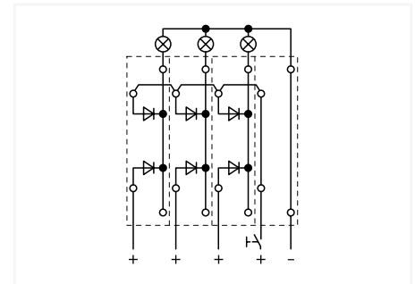
Lamp test circuits can be created using the following terminal blocks: 870-542/281-487 or 870-542/281-488
